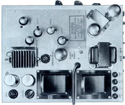
Dynatone Amplifier
