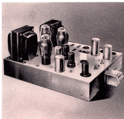
SIMPLIFIED AMPLIFIER AND JUNCTION BOX
